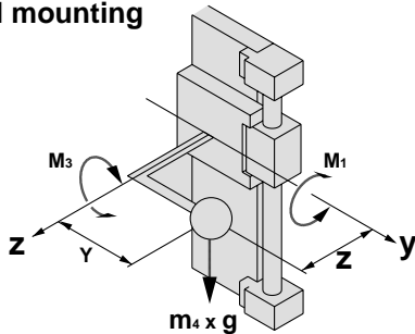
Vertical mounting
