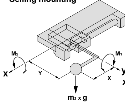
Ceiling mounting
