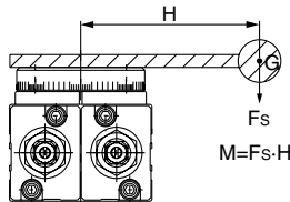
Vertical Mounting
