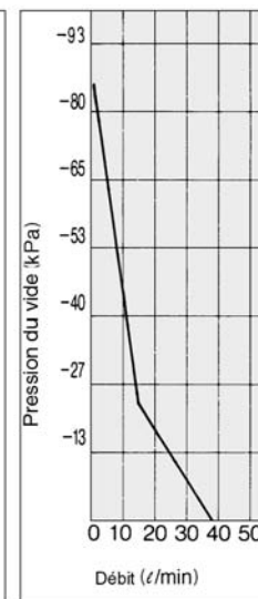
Flow characteristics
