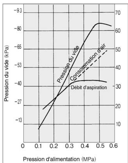
Exhaust characteristics
