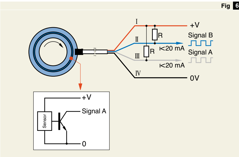
Circuit diagram
