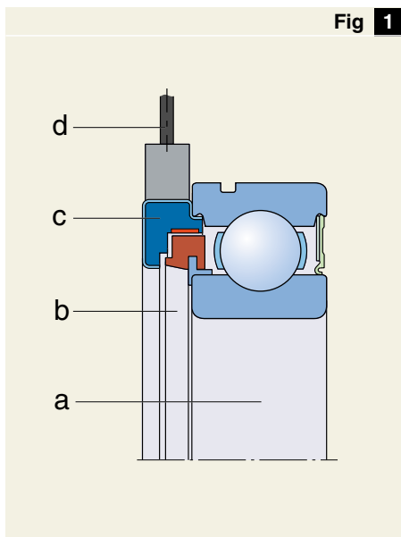
Components of SKF Sensor-Bearing Unit
