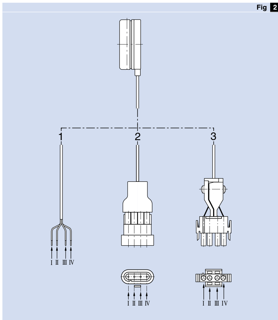
Components of SKF Sensor-Bearing Unit
