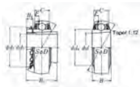
UKX...D1;H, HA, HE, HS
