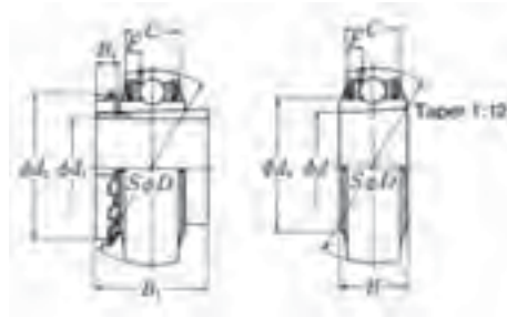
UK2...D1;H, HA, HE, HS
